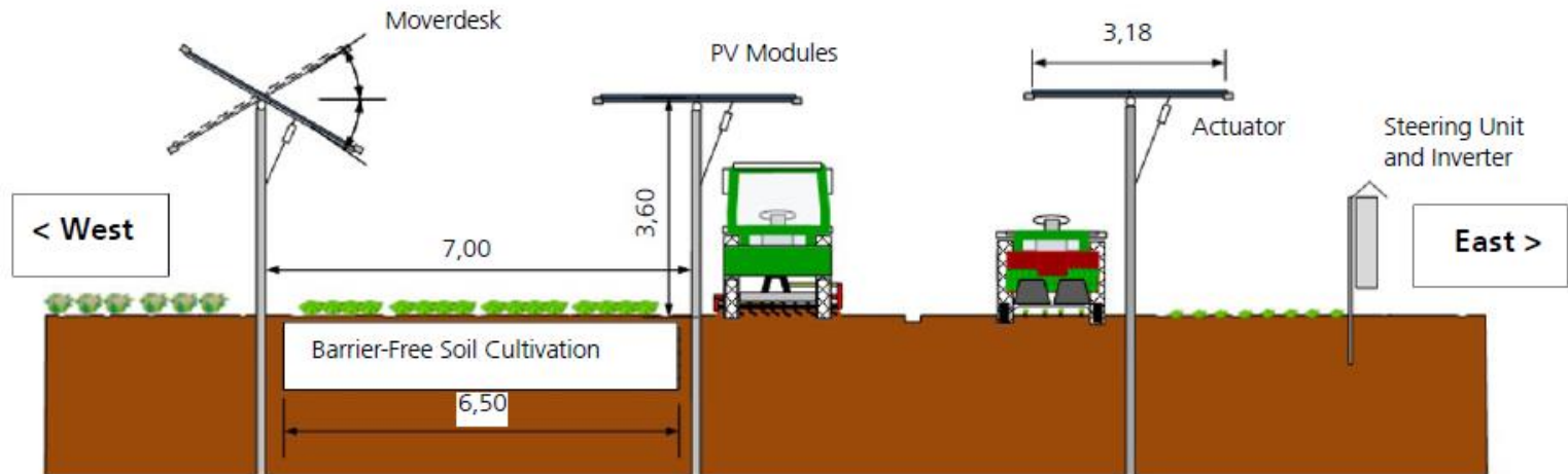
Figure 9: Cross-section of the agrivoltaic plant in Weißenstephan. © 2020 B. Ehrmaier, M. Beck, U. Bodmer
